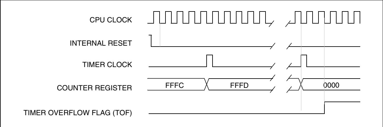
Figure 46. Counter Timing Diagram, Internal Clock Divided By 8
